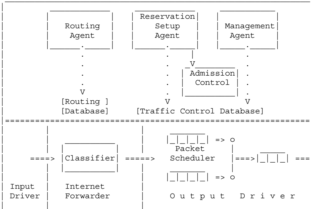
Figure 1: Implementation Reference Model for Routers
