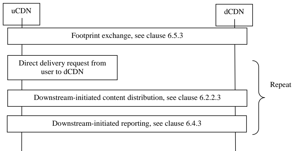
Figure C.4.1: Scenario for managed delivery of content.
