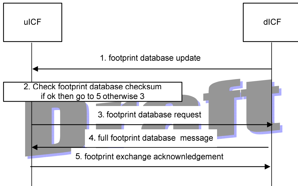
Figure 6.5.3.1: Footprint Exchange
