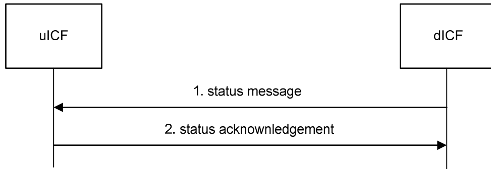
Figure 6.5.4.1: Service Status Exchange
