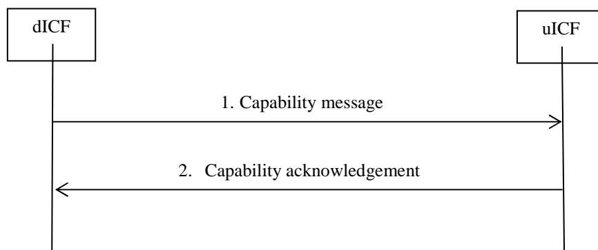
Figure 6.5.2.1: Capability Exchange
