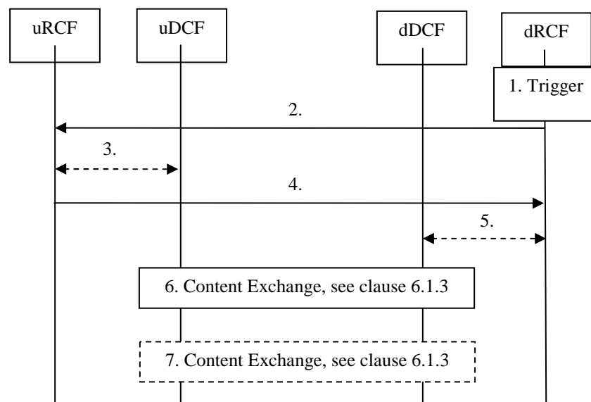
Figure 6.2.2.3.1: Downstream-initiated content distribution
