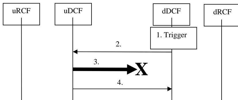
Figure 6.2.3.4.1: Stream release
